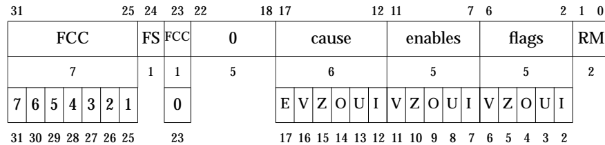
Figure B-14 MIPS IV - FPU Control and Status Register (FCSR)
