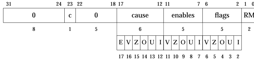
Figure B-13 MIPS III - FPU Control and Status Register (FCSR)
