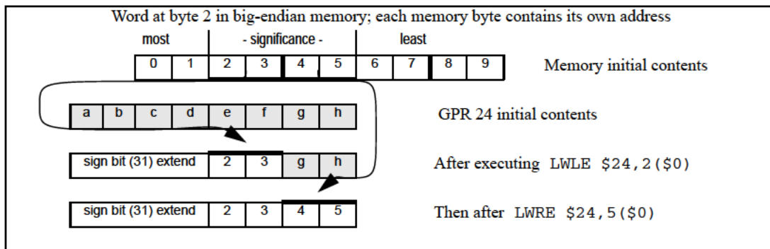
Figure 3.18 Unaligned Word Load Using LWLE and LWRE
