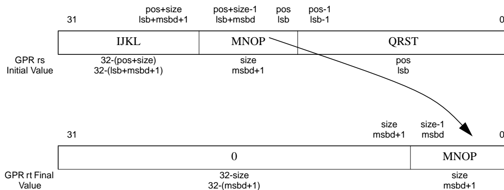
Figure 3.10 Operation of the EXT Instruction
