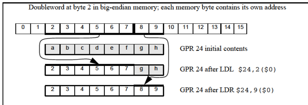
Figure 3.14 Unaligned Doubleword Load Using LDR and LDL
