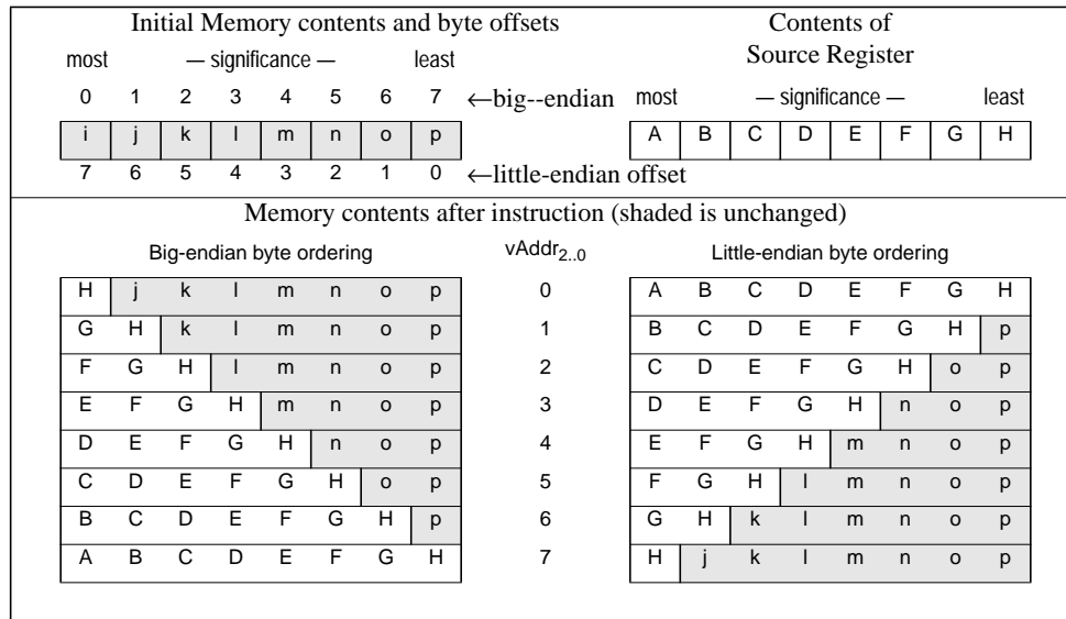
Figure 4.27 Bytes Stored by an SDR Instruction
