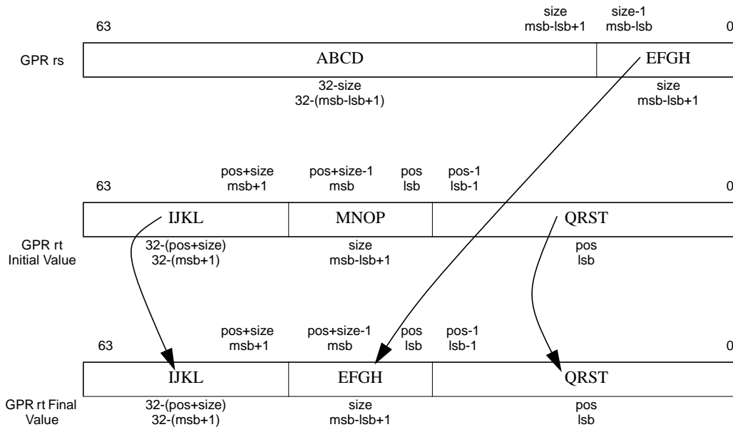
Figure 3.9 Operation of the DINSU Instruction
