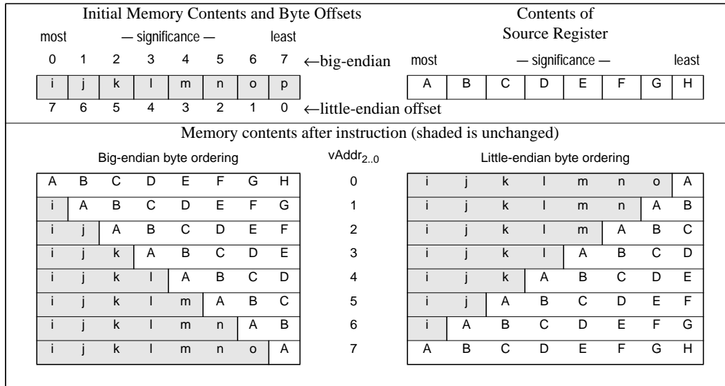
Figure 4.25 Bytes Stored by an SDL Instruction
