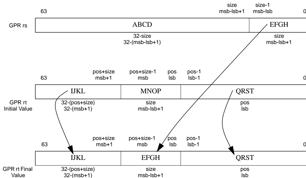
Figure 3.8 Operation of the DINSM Instruction
