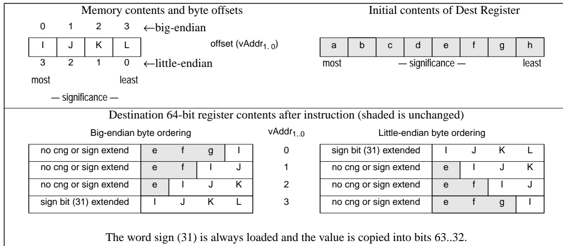
Figure 3.21 Bytes Loaded by LWR Instruction
