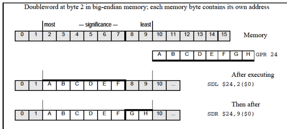
Figure 4.24 Unaligned Doubleword Store With SDL and SDR
