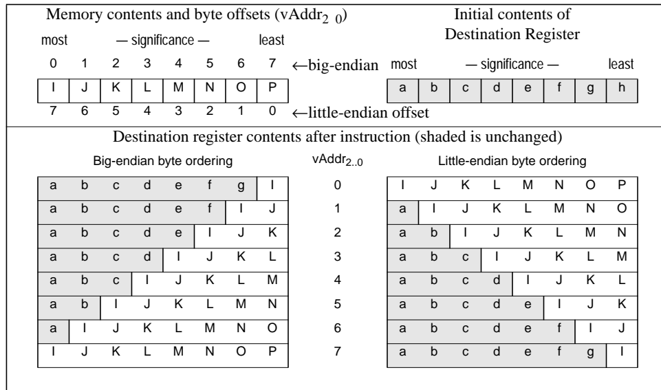
Figure 3.15 Bytes Loaded by LDR Instruction
