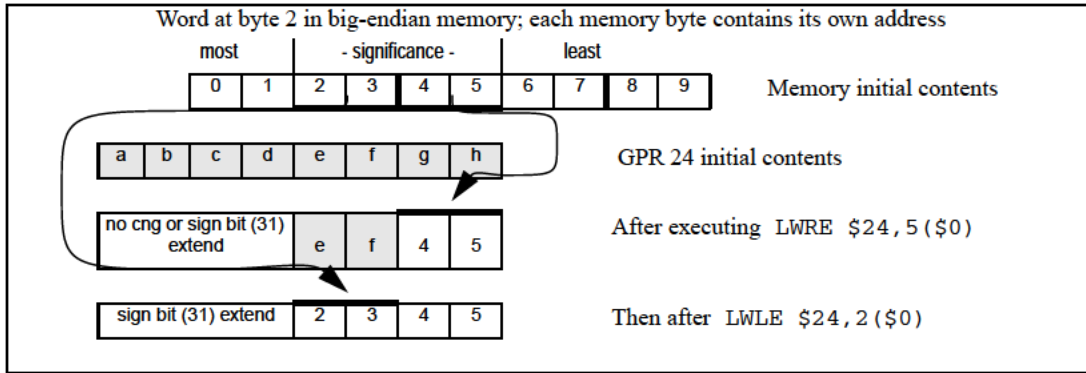
Figure 3.22 Unaligned Word Load Using LWLE and LWRE
