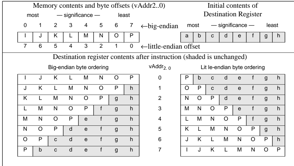
Figure 3.13 Bytes Loaded by LDL Instruction
