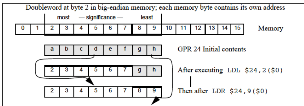
Figure 3.12 Unaligned Doubleword Load Using LDL and LDR
