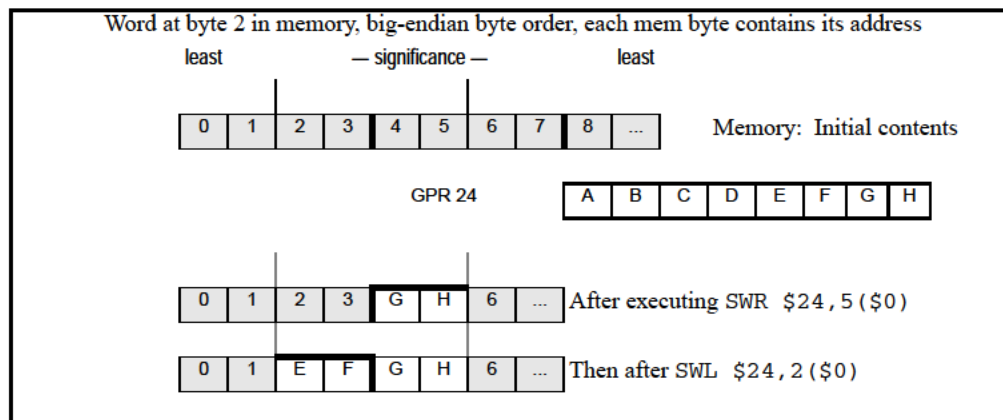
Figure 4.32 Unaligned Word Store Using SWR and SWL
