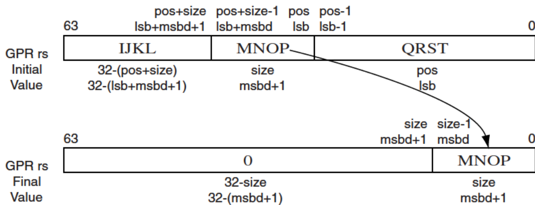
Figure 3.4 Operation of the DEXT Instruction
