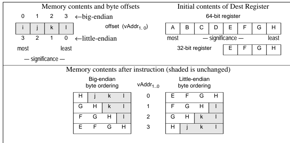
Figure 4.35 Bytes Stored by SWRE Instruction
