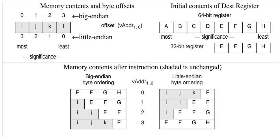
Figure 4.31 Bytes Stored by an SWLE Instruction
