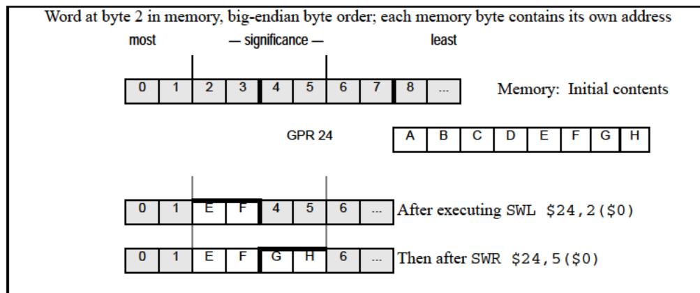
Figure 4.28 Unaligned Word Store Using SWL and SWR
