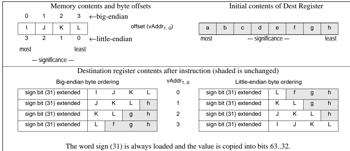
Figure 3.19 Bytes Loaded by LWLE Instruction
