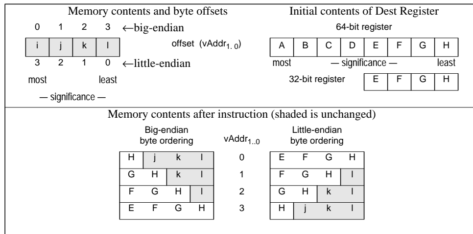
Figure 4.33 Bytes Stored by SWR Instruction
