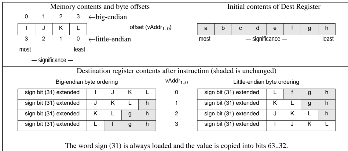
Figure 3.17 Bytes Loaded by LWL Instruction
