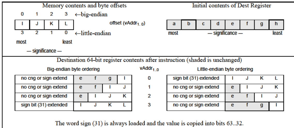
Figure 3.23 Bytes Loaded by LWRE Instruction
