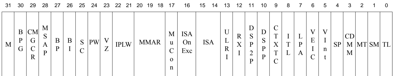
Figure 9-47 Config3 Register Format
