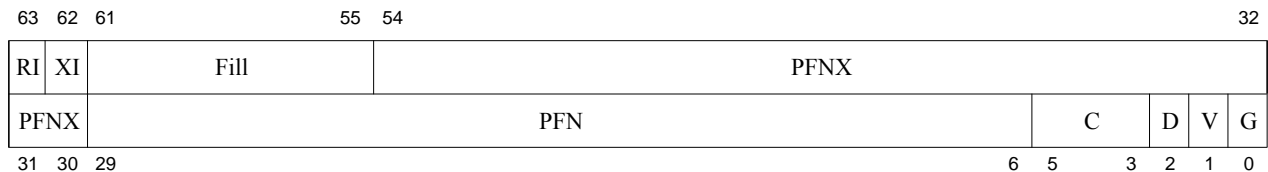
Figure 9-5 EntryLo0, EntryLo1 Register Format in Release 3 of the Architecture when Accessed with DMFC0 &amp; DMTC0 Instructions
