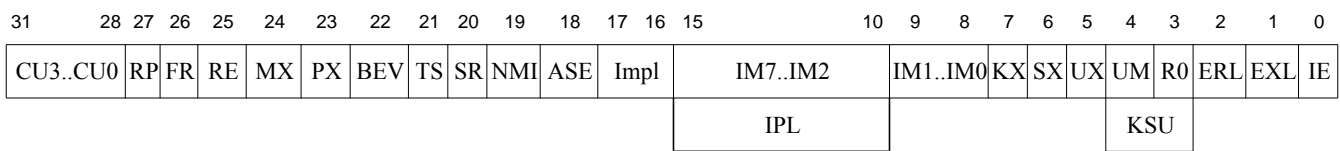
Figure 9.31 Status Register Format
