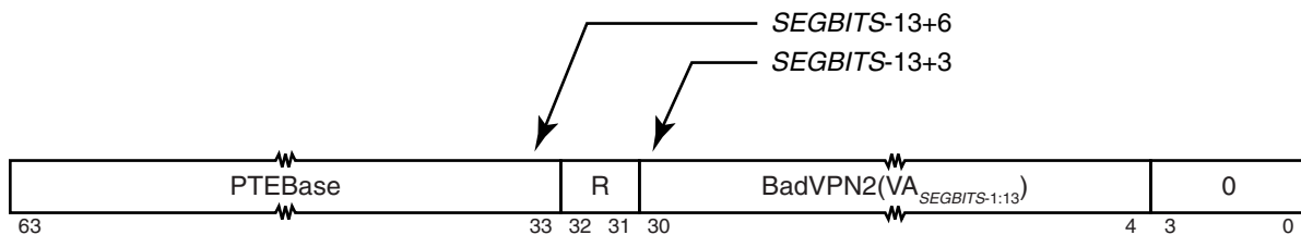
Figure 9.54 XContext Register Format when Config3_{CTXTC} = 0
