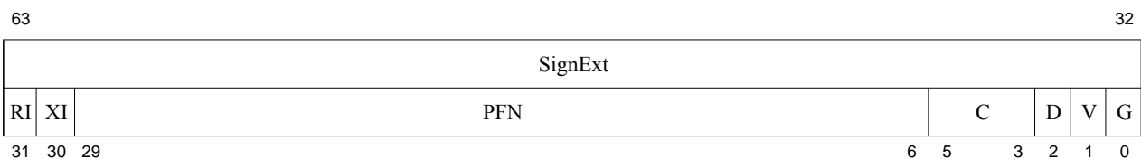
Figure 9-6 EntryLo0, EntryLo1 Register Format in Release 3 of the Architecture when Accessed using MFC0 and MTC0 Instructions
