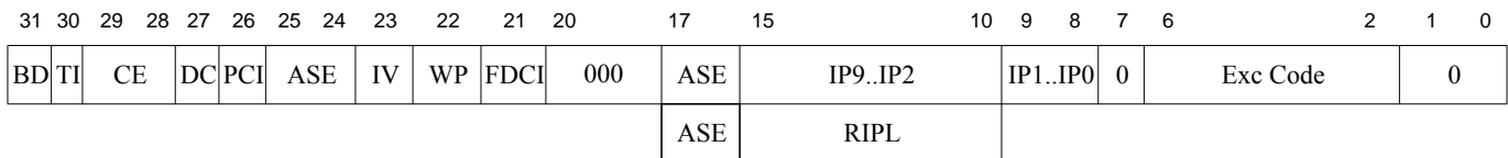
Figure 9.35 Cause Register Format
