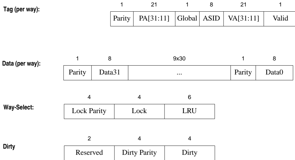
Figure 9.2 Data Cache Organization
