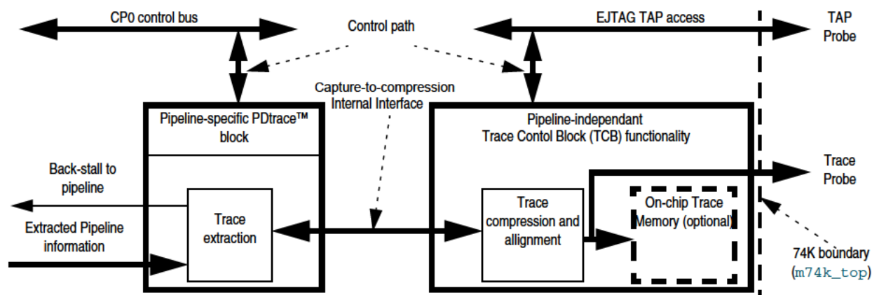
Figure 11.30 MIPS® Trace Functional Blocks in the 74K™ Core
