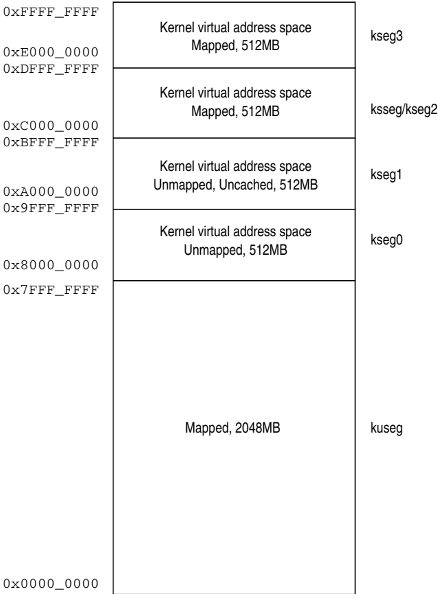
Figure 5.6 Kernel Mode Virtual Address Space
