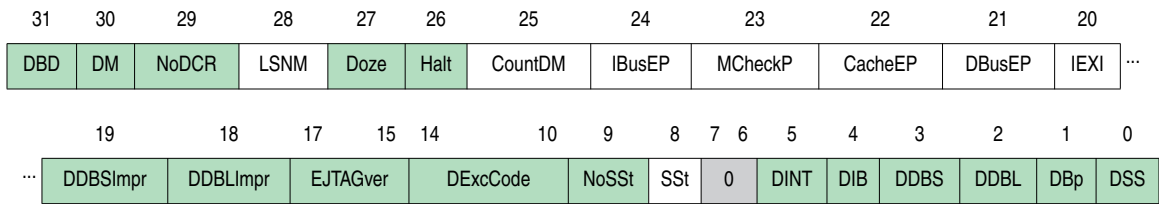
Figure 7.32 Debug Register Format
