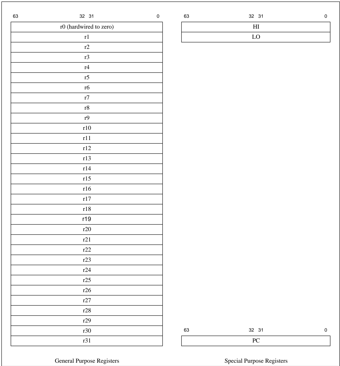
Figure 2.8 CPU Registers
