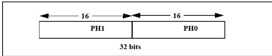
Figure 7.3 The Little-Endian PH0 and PH1 Elements in a GPR for the microMIPS32 Architecture
