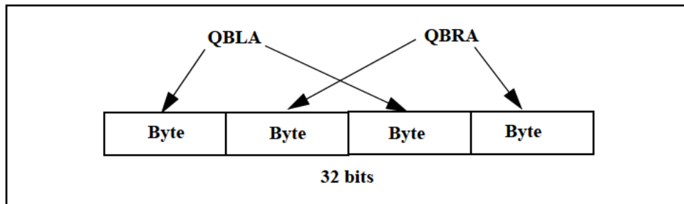
Figure 7.5 The Endian-Independent QBLA and QBRA Elements in a GPR for the microMIPS32 Architecture
