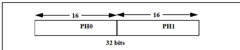
Figure 7.2 The Big-Endian PH0 and PH1 Elements in a GPR for the microMIPS32 Architecture
