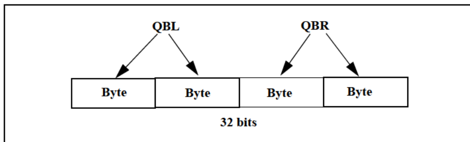
Figure 7.4 The Endian-Independent QBL and QBR Elements in a GPR for the microMIPS32 Architecture
