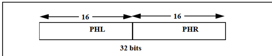
Figure 7.1 The Endian-Independent PHL and PHR Elements in a GPR for the microMIPS32 Architecture
