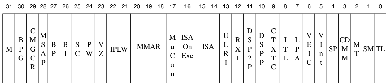
Figure 5-9 Config3 Register Format
