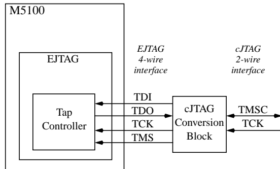
Figure 8 cJTAG Support
