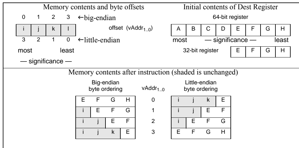
Figure 6.18 Bytes Stored by an SWL Instruction
