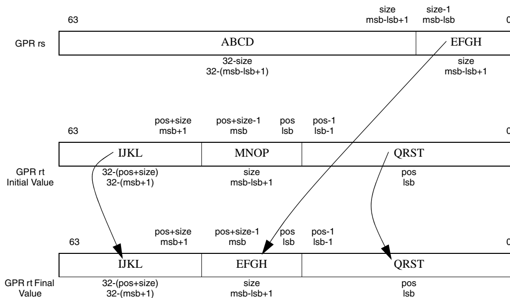
Figure 3.10 Operation of the DINSM Instruction
