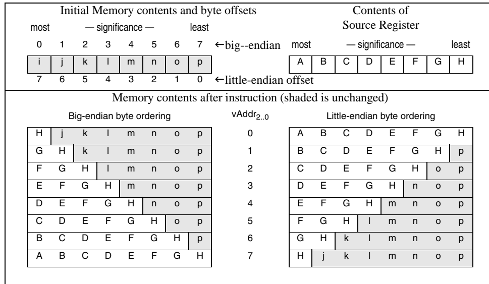
Figure 6.16 Bytes Stored by an SDR Instruction
