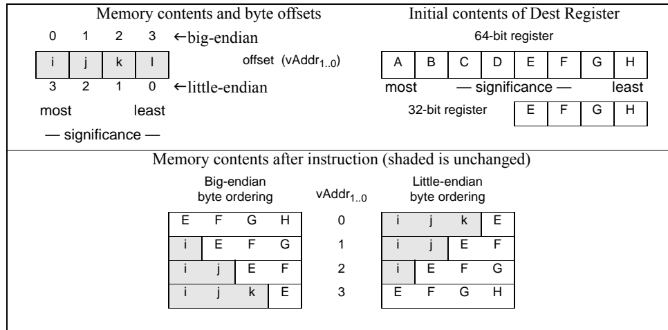
Figure 6.20 Bytes Stored by an SWLE Instruction
