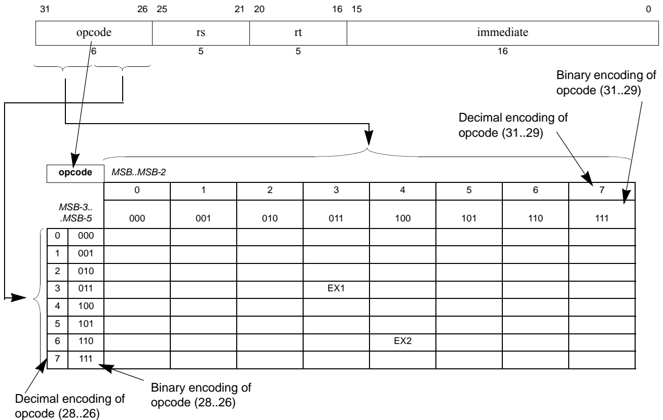
Figure 11.1 Sample Bit Encoding Table
