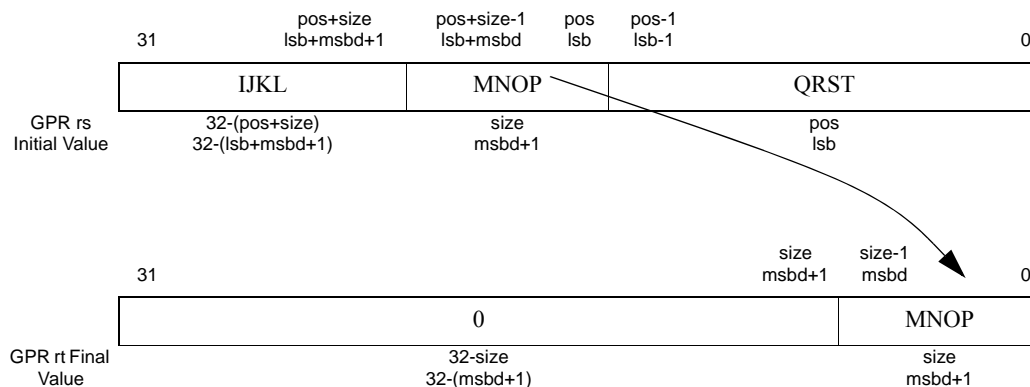
Figure 5.11 Operation of the EXT Instruction
