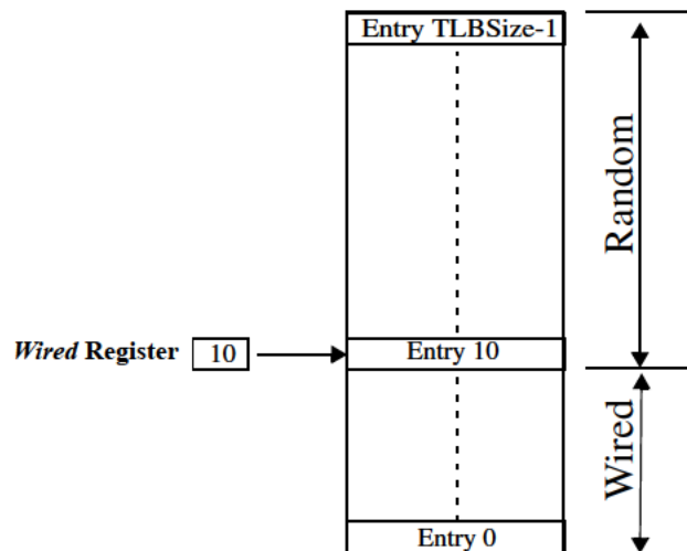
Figure 9.23 Wired And Random Entries In The TLB
