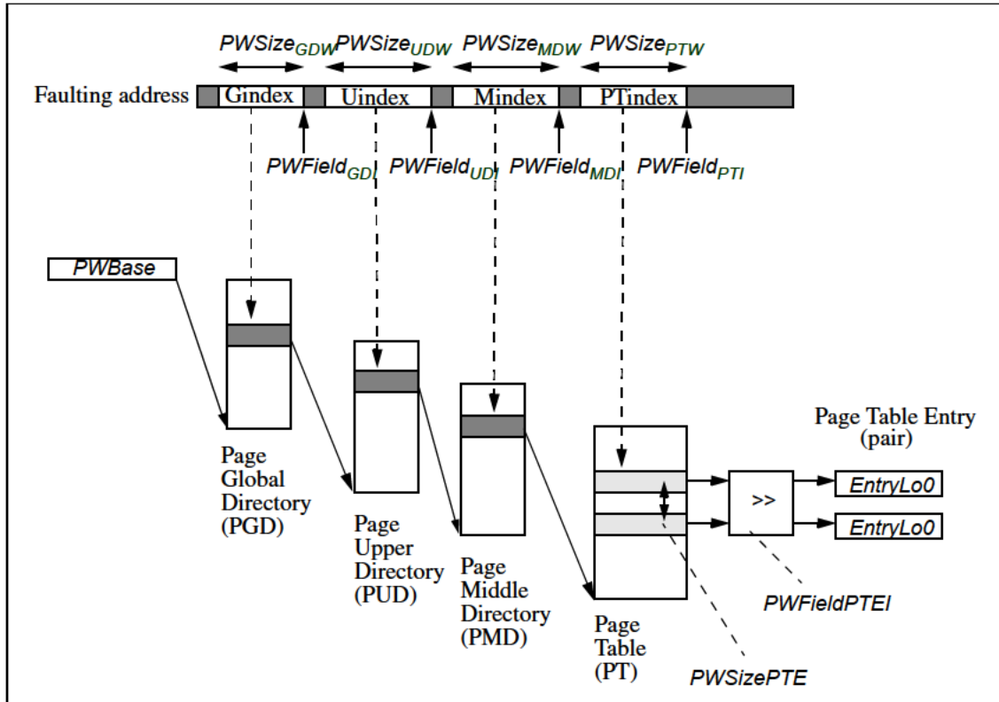
Figure 4.8 Page Table Walk Process & CP0 Control fields
